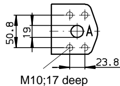
Detail W
