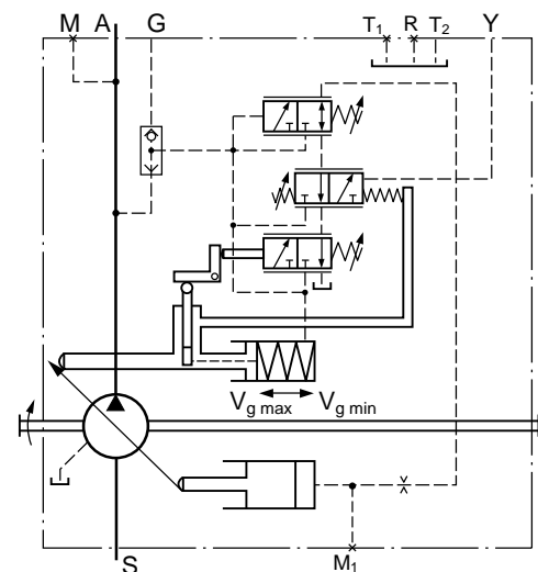
Constant power control with pressure cut-off and hydraulic stroke limiter, LRDH1, LRDH5 (Function: V_{g \max} to V_{g \min} )
