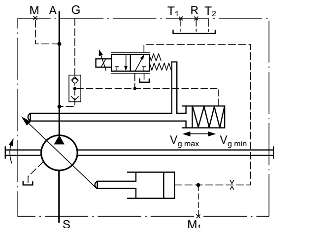
Electrical control with proportional solenoid, EP
