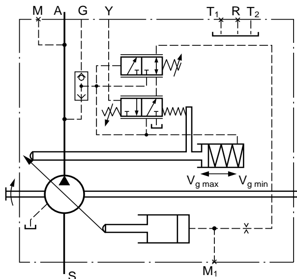
Hydraulic control, pilot pressure related, with integral pressure cut-off (fixed setting), HD1D, HD2D
