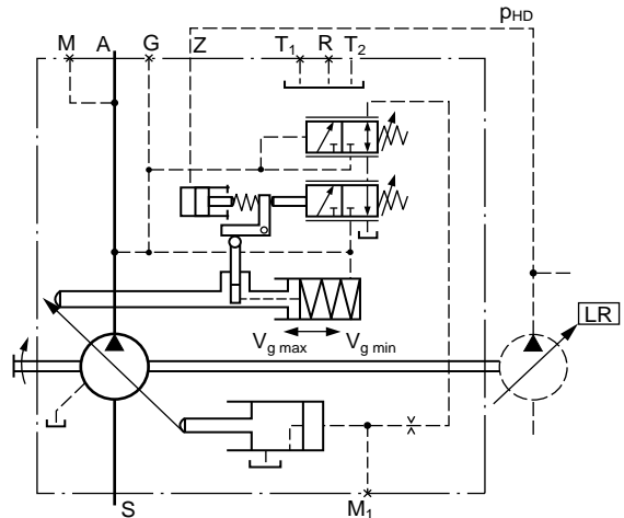
Power control with pressure cut-off and cross sensing control, LRCD
