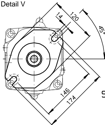
Detail V
