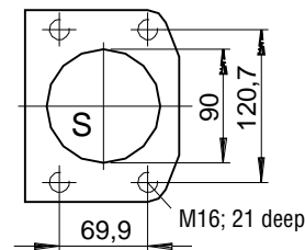
Detail W
