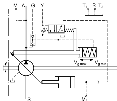
Hydraulic control, pilot pressure related, HD1, HD2
