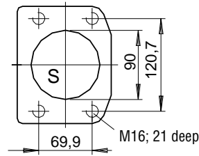
Detail W
