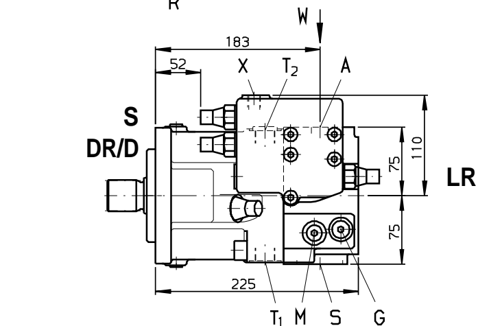
Detail W
