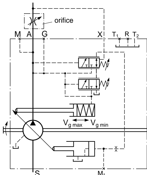
Constant pressure control with load sensing valve, DRS
